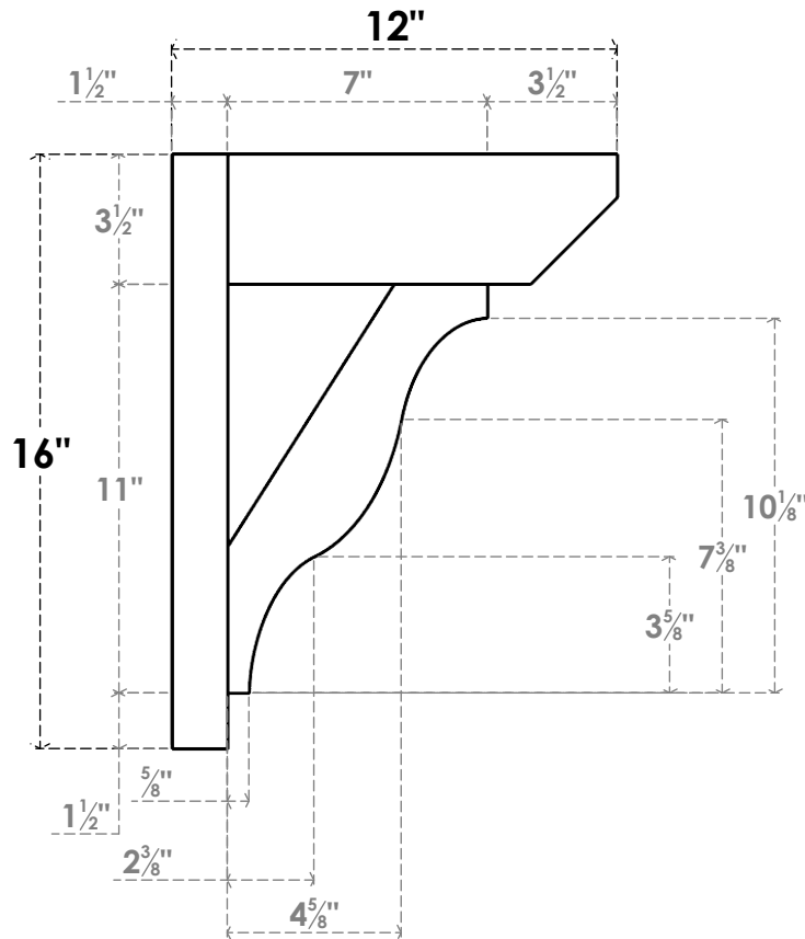
SIDE PROFILE
